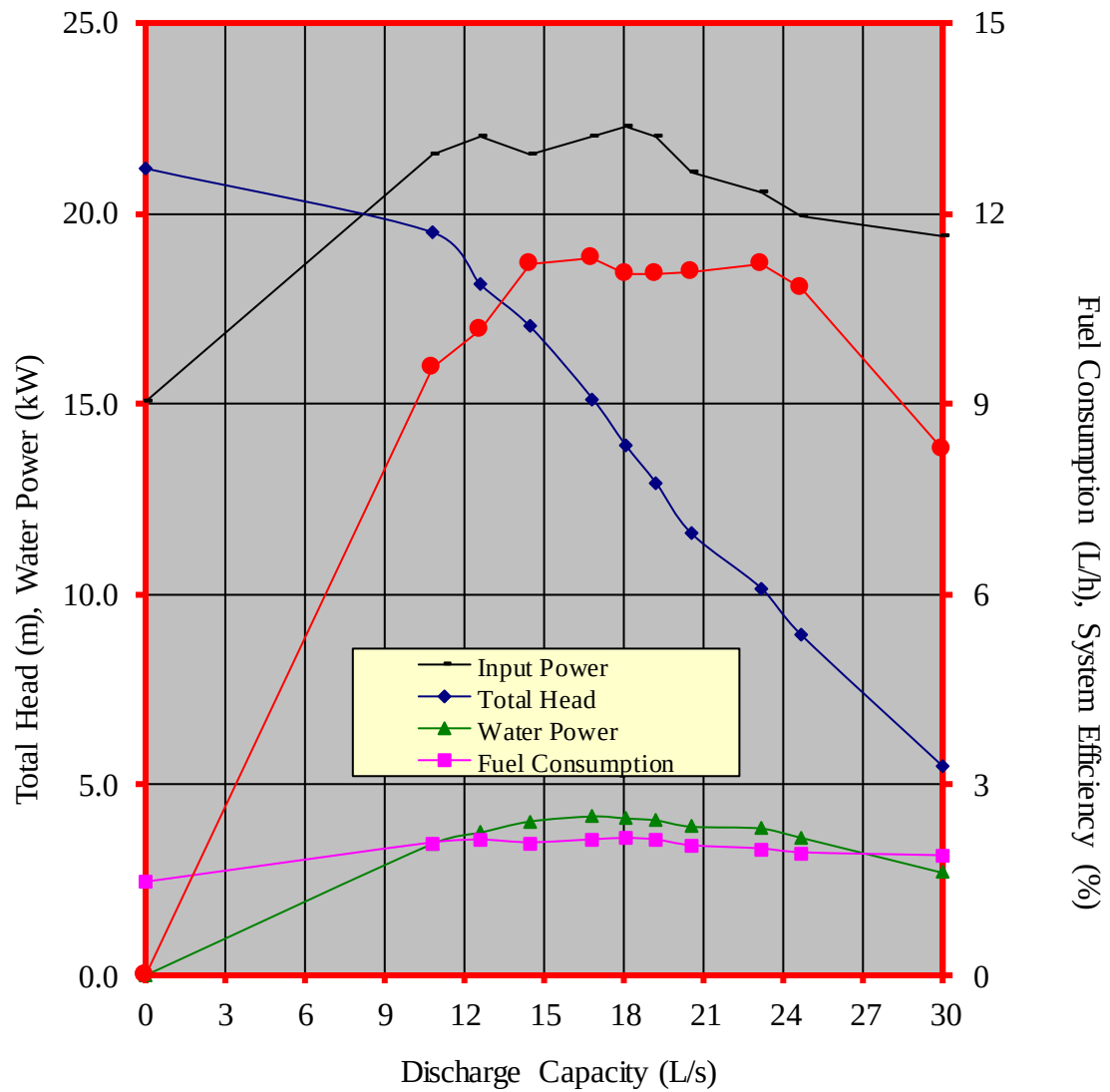
Figure 3. Performance characteristic curves of the EAGLE EC-100(4") coupled to KUBOTA RK 80-1S diesel engine centrifugal pump
